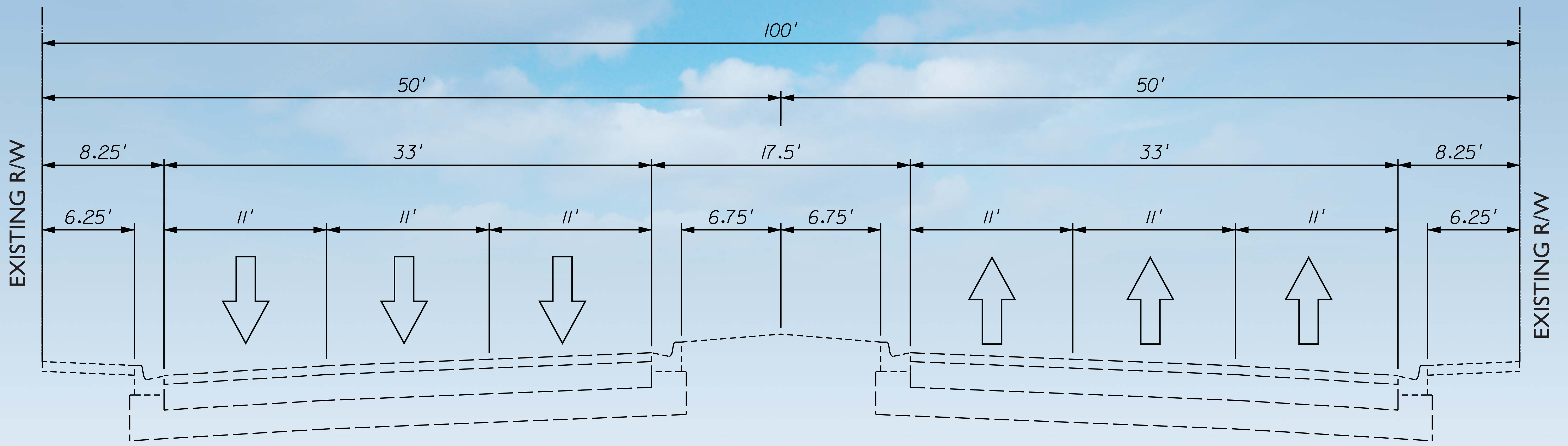
Existing Typical Section (from NW 27th Ave to NW 7th Ave)
